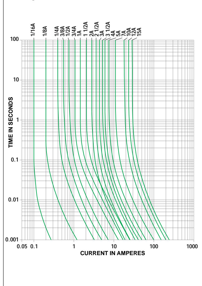
Average Time Current Curves
